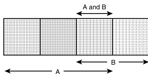
Figure 17-1 Conditional Probabilities in Bayes' Theorem
